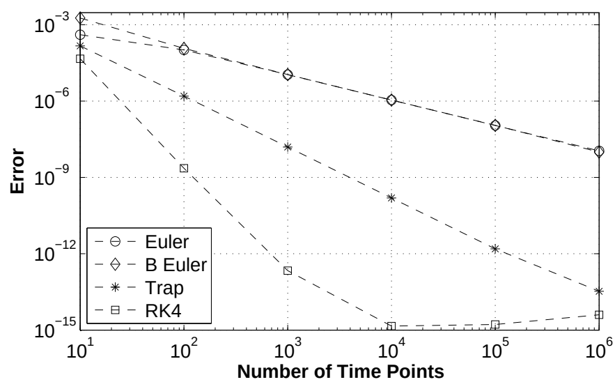
Figure 1: Logistic Equation
